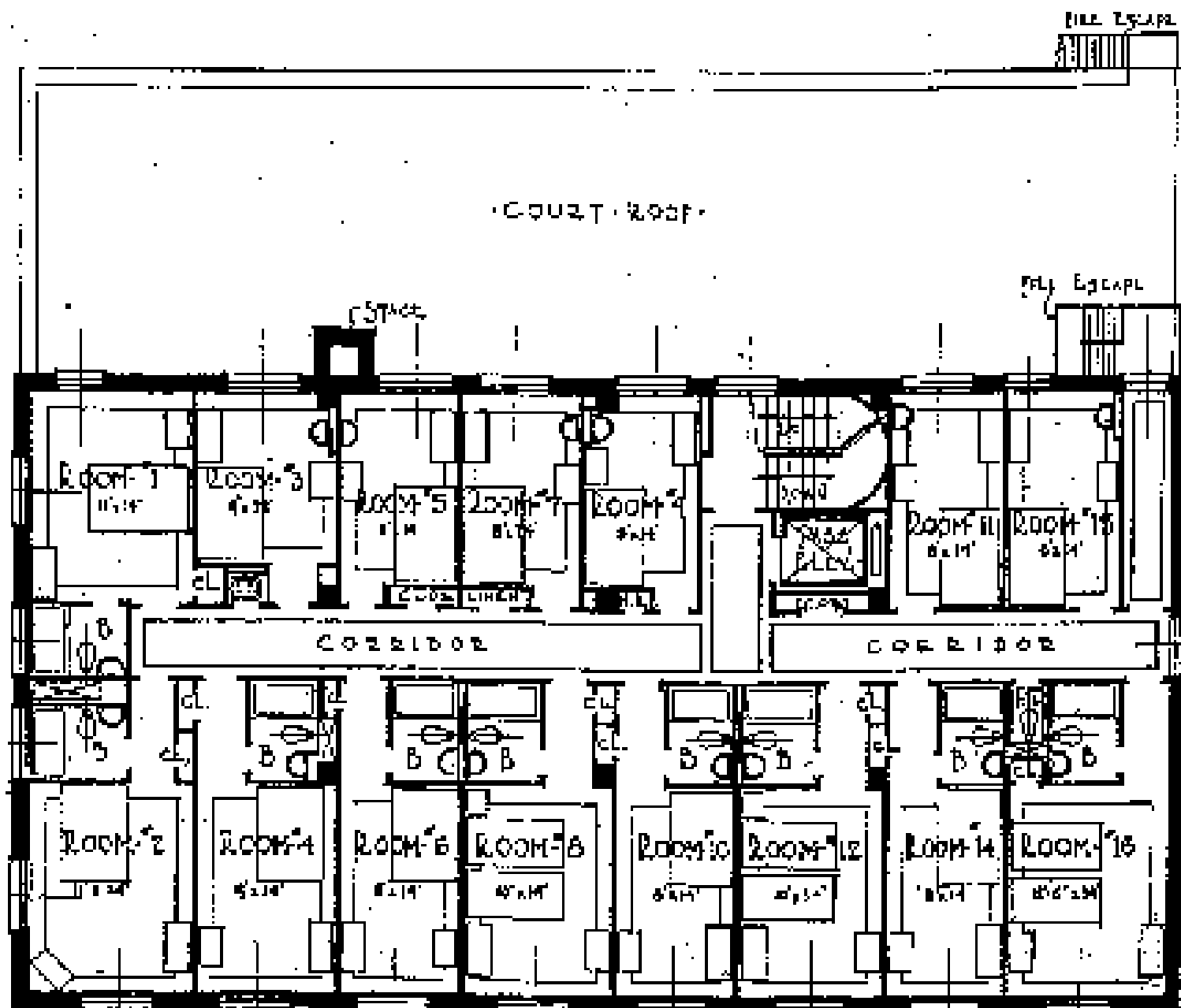
Typical floor plan Hotel Franklin, West, Ohio, H. M. Stevens & Son, architects.
